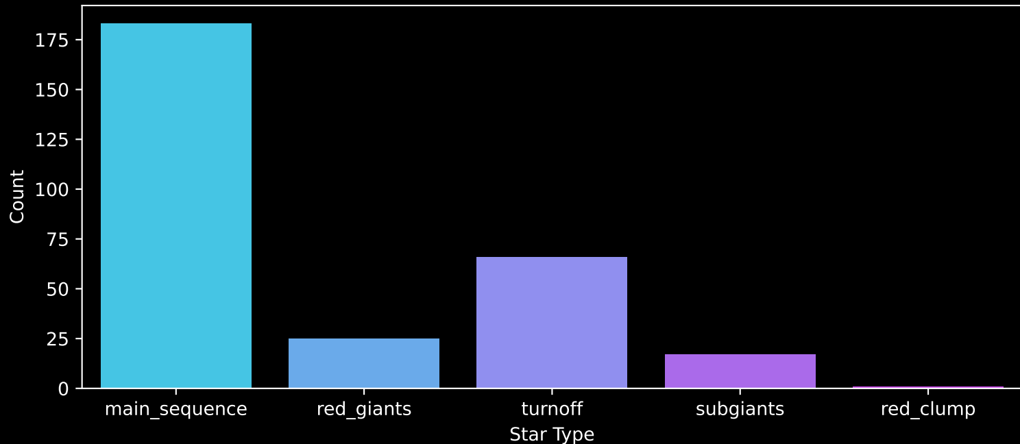
GALAH DR4 Field: [6861] Count plot of Star Type
