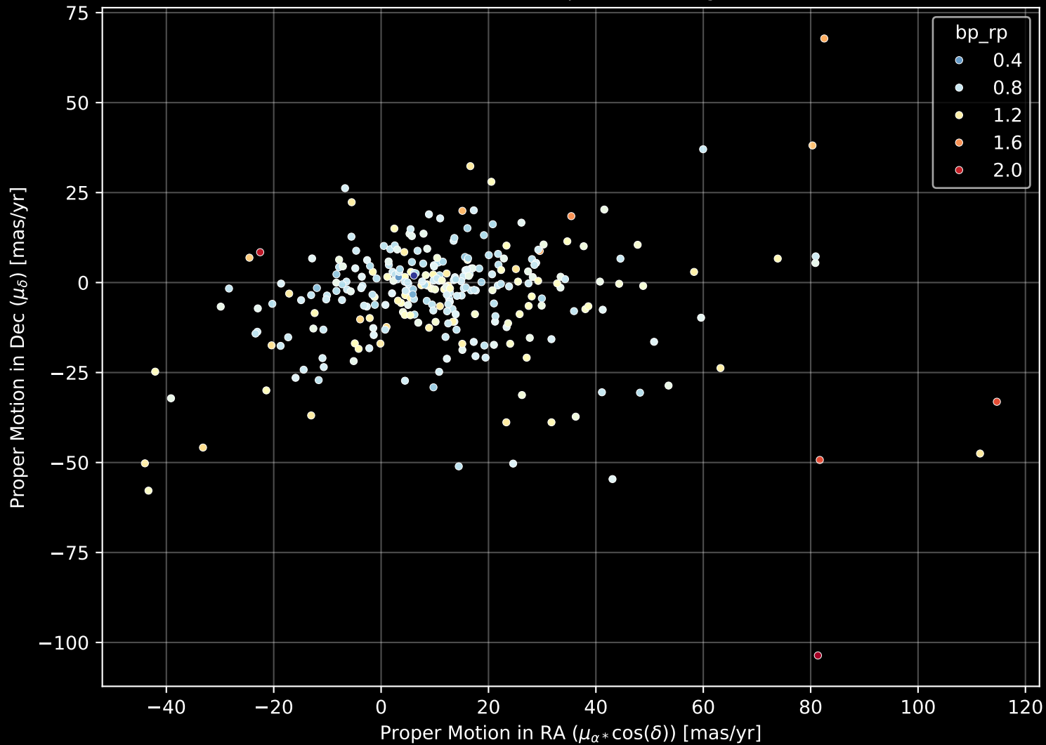
GALAH DR4 Field: [6861] Proper Motion Diagram (n= 292)
