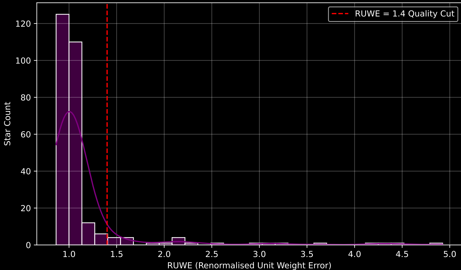
GALAH DR4 Field [6861] RUWE Distribution (n= 277)
