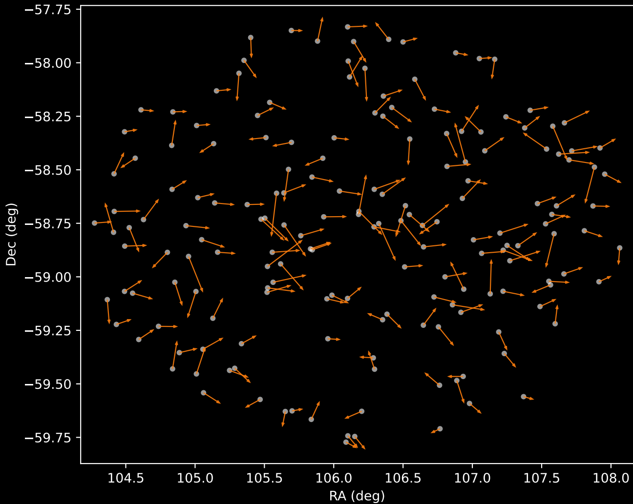
GALAH DR4 Cluster 2 Proper Motion Vectors (n=174)
